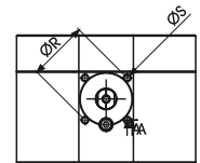
HOLE FOR ACTUATOR ISO5211
